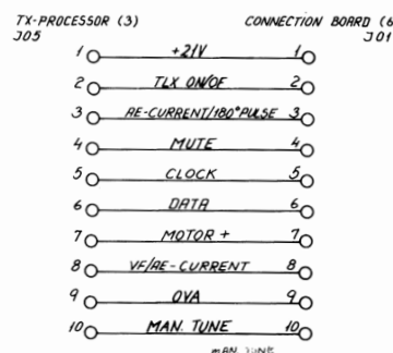
CABLE 3 : TX-PROCESSOR TO CONNECTION BOARD
