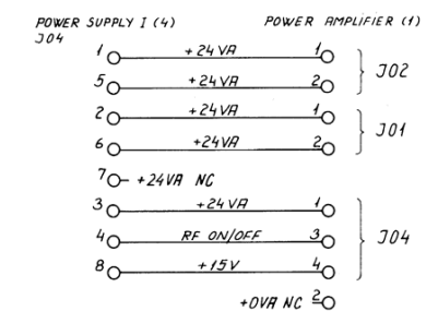
CABLE 7 : POWER SUPPLY I TO POWER AMPLIFIER
